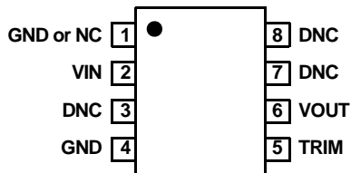
ISL21007 (8 LD SOIC) TOP VIEW
